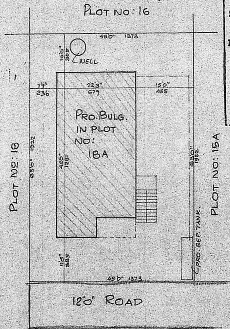
SITE PLAN
